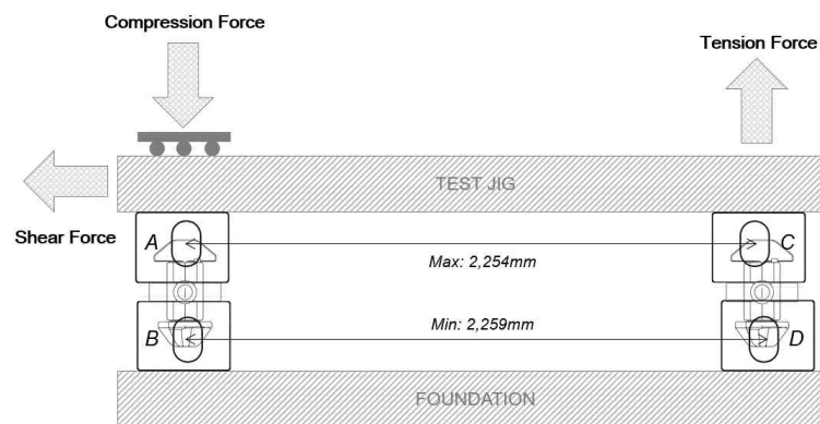
Fig. 3.25.3 Configuration of HHS test equipment (semi-automatic twistlock) (2021)
