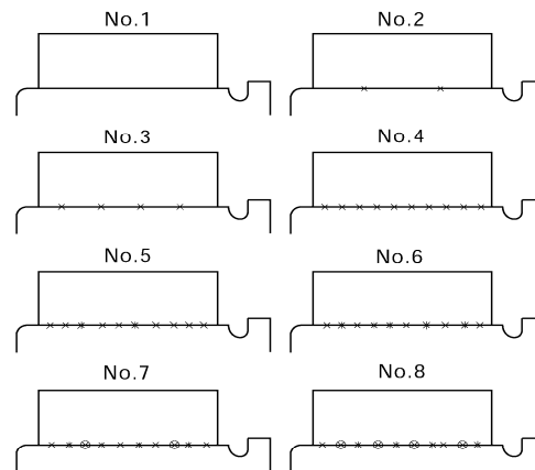
Fig 6.1.3 spark on surface of commutator
