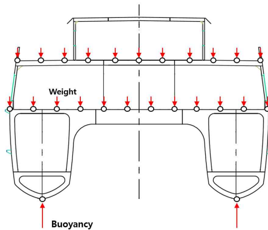
Figure 3.1.3 An example for application of weight and buoyancy
