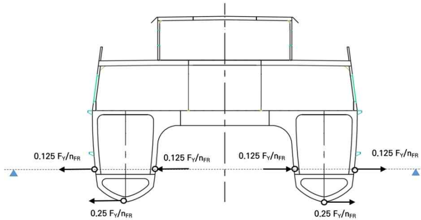
Figure 3.1.4 Application of horizontal split force for transverse bending moment ( n_{FR} is no. of frames)
