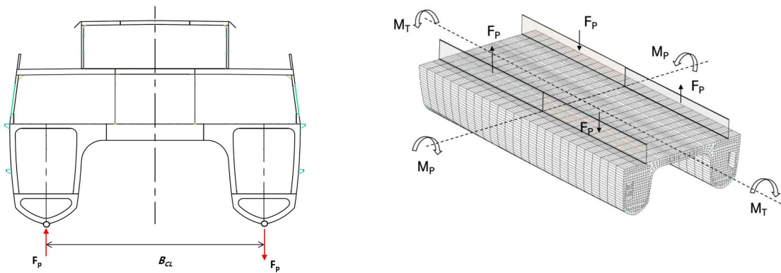
Figure 3.1.5 Application of pitch connecting force for longitudinal/transverse torsional moment
