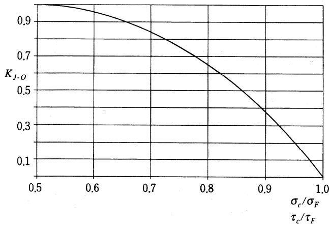
Fig 3.1 Factor K_{J-0}
