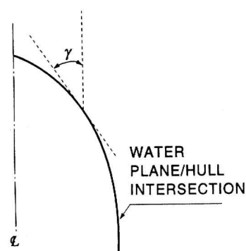
Fig 3.2.7 Angle \gamma
