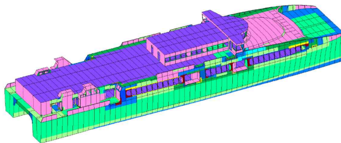
Figure 3.1.1 An example of the full ship structural model
