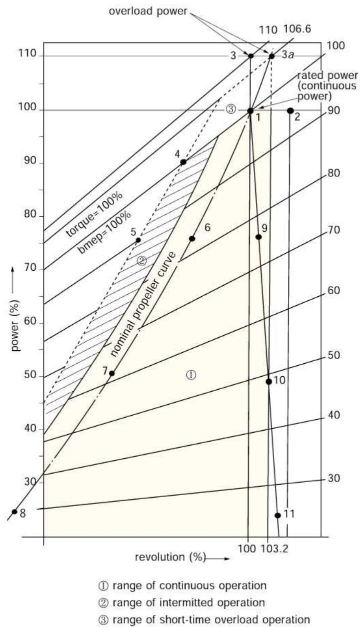
Fig 3.8.1 Power/Revolution Diagram
