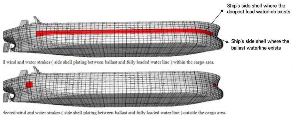
Fig 1.2.6 Wind and Water Strakes (from the IACS Rec. 96)
