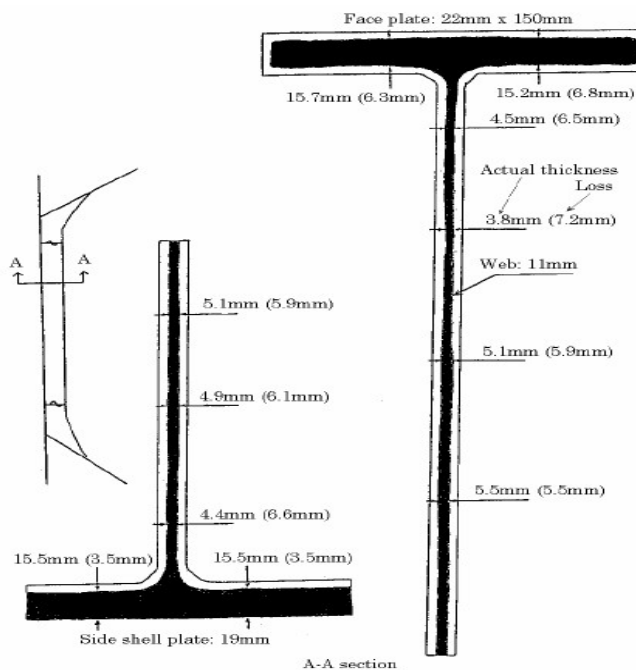
Fig. 1.2.2 General corrosion (from IACS Rec. 76)
