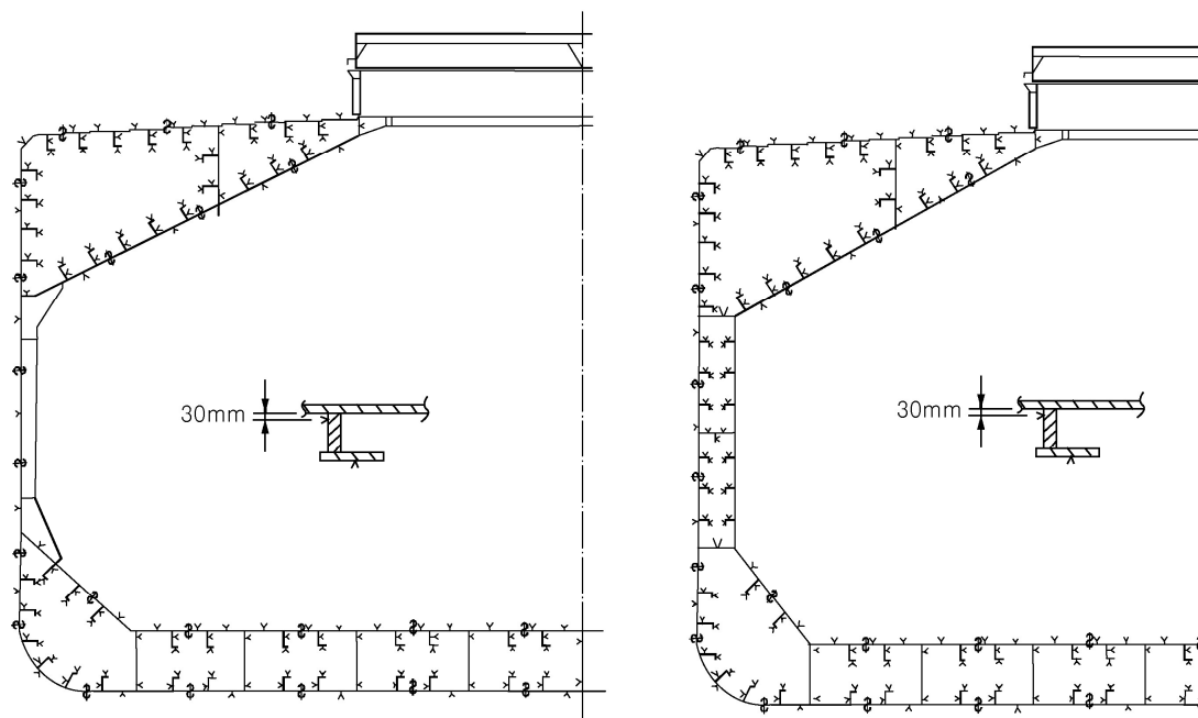
Fig 3 Locations of measurements on transverse section of single skin or double skin bulk carrier
