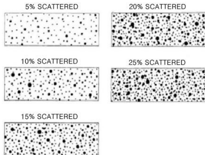
Fig 1.2.3 Pitting intensity diagrams
