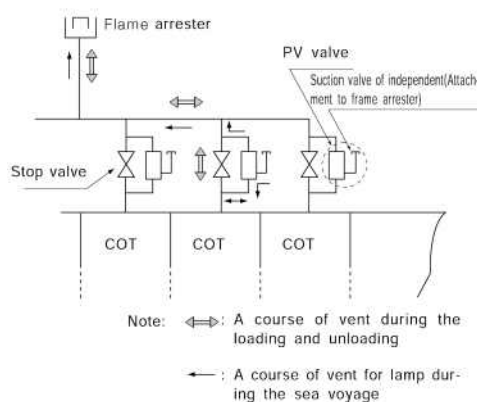
Fig. 8.2.8 Examples of isolation of cargo oil tank
