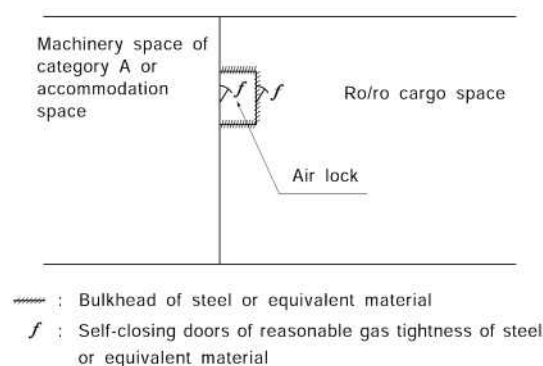
Fig 8.13.2 Air lock (2017)
