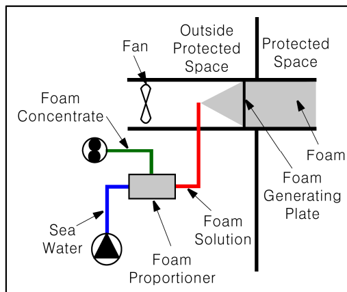
Fig 8.8.5(Outside air supply type)
