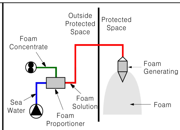
Fig 8.8.6(Inside air supply type)
