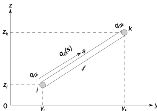
Figure 1 : Definition of line segment
