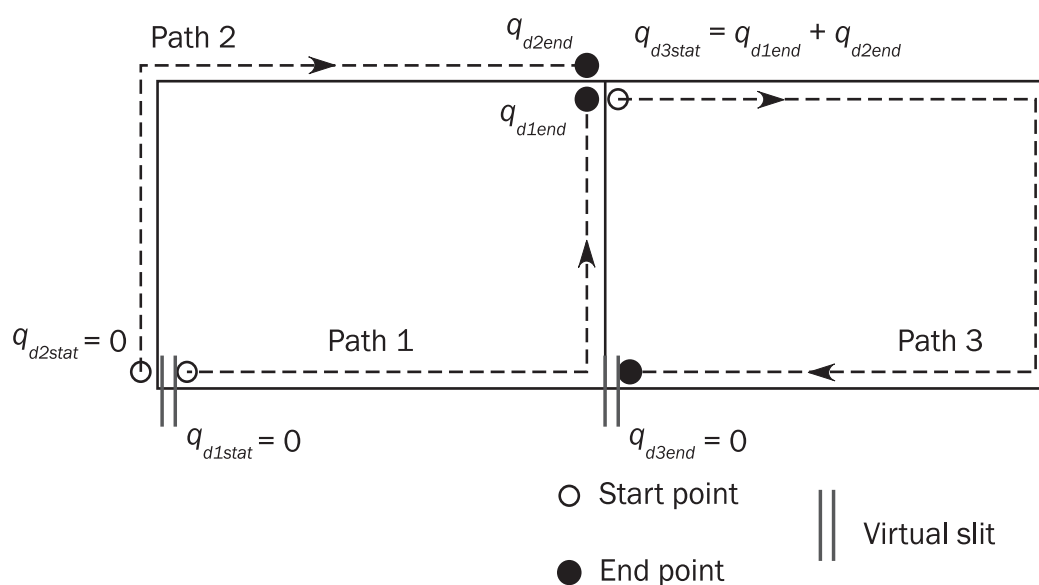
Figure 2 : Calculation of determinate shear flow at bifurcation
