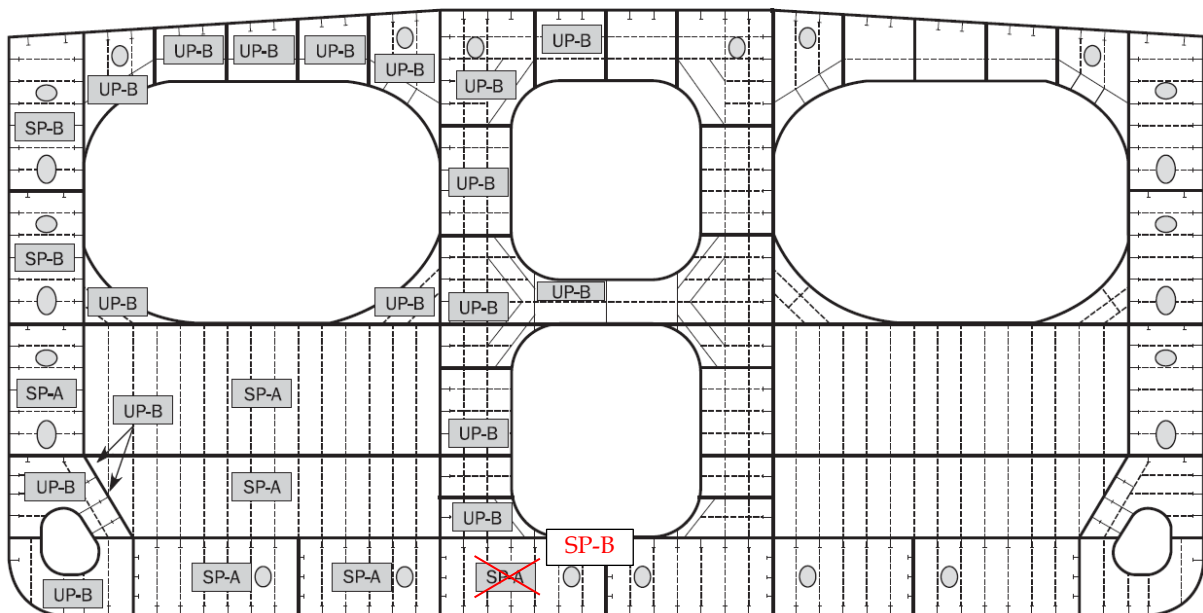
Figure 4 : Cross tie
