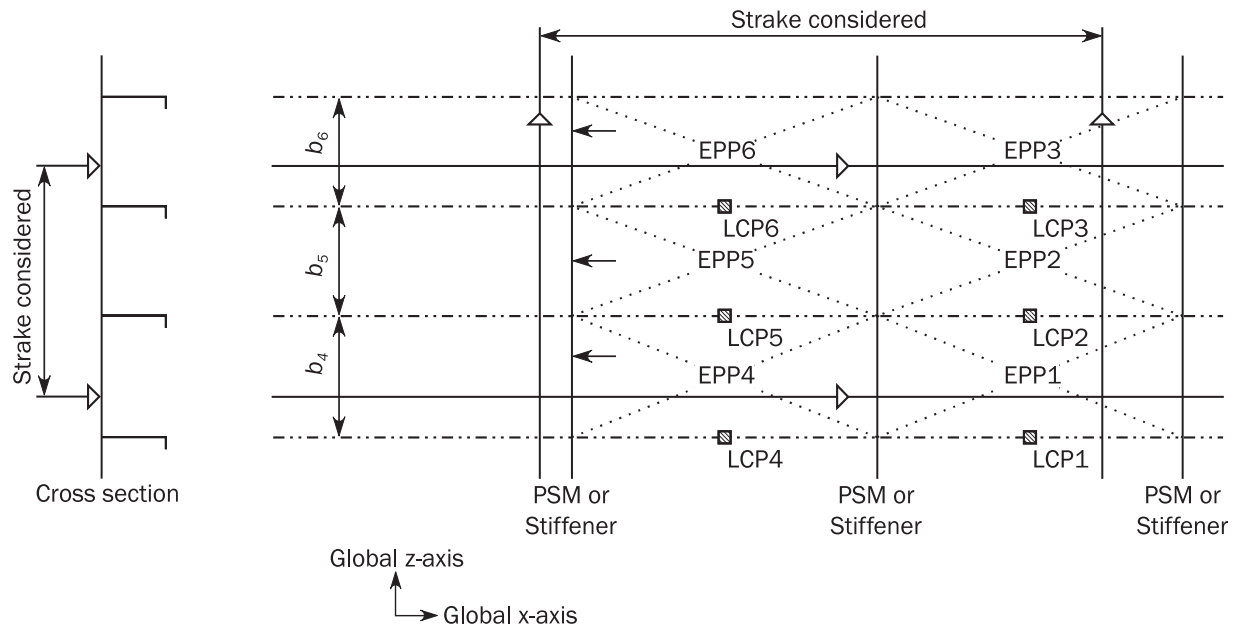
Figure 19 : Load calculation point for transverse framing
