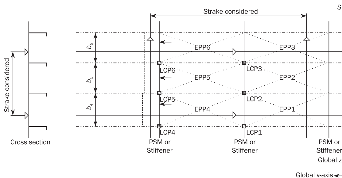
Figure 21 : Load calculation point for vertical framing on transverse vertical structure
