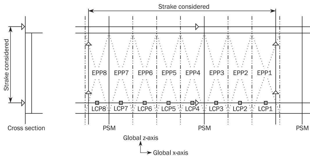
Figure 19 : Load calculation point for transverse framing
