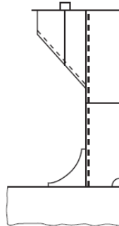
5 Figure 4 : Coaming stay (example 2)
