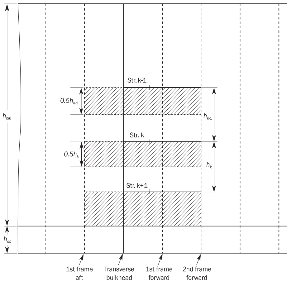
Figure 8 : Region for stringer correction, t_p , for ships with 3 stringers
