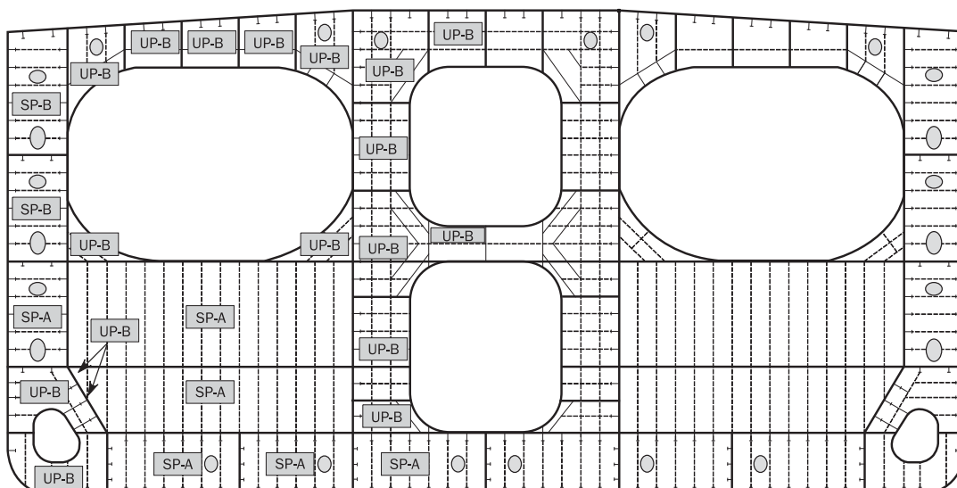
Figure 4 : Cross tie
