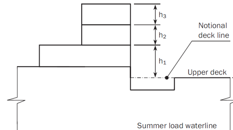
Figure 1 : Measurement of heights
